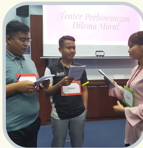
2. Lakonan anti-model
